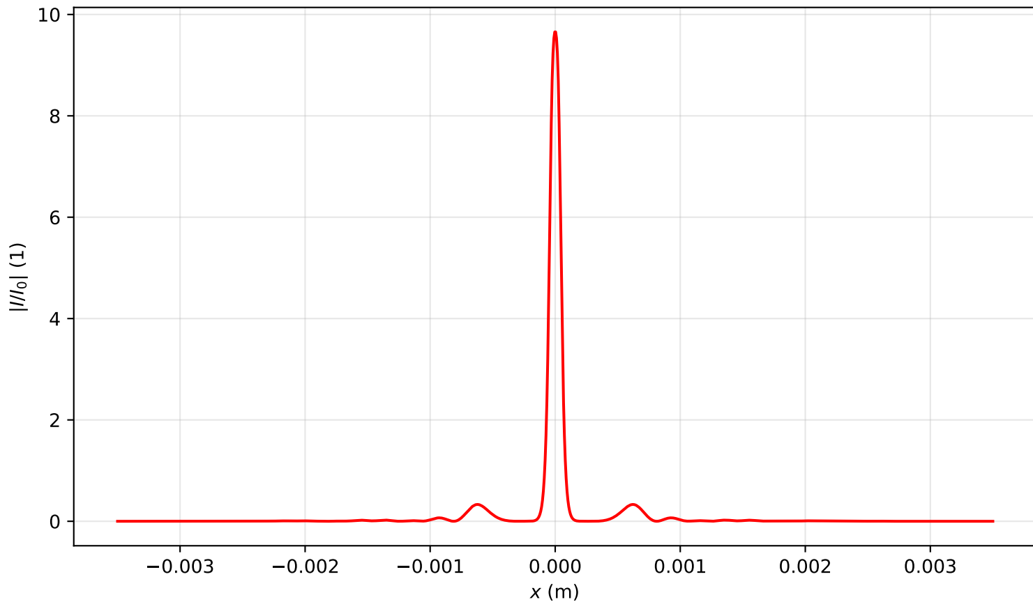
Intensity profile I(x, y = 0, z = 0.478)/I_0 , P_{in}=7.0P_{cr} , artificial time
